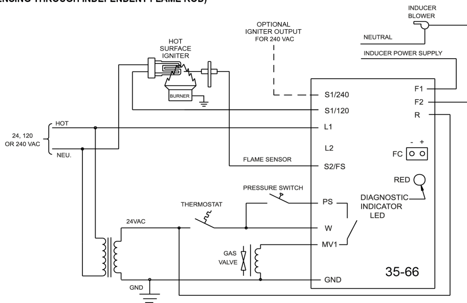
Figure 2. Remote Sense
